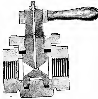
Fig. 2981. Section.
